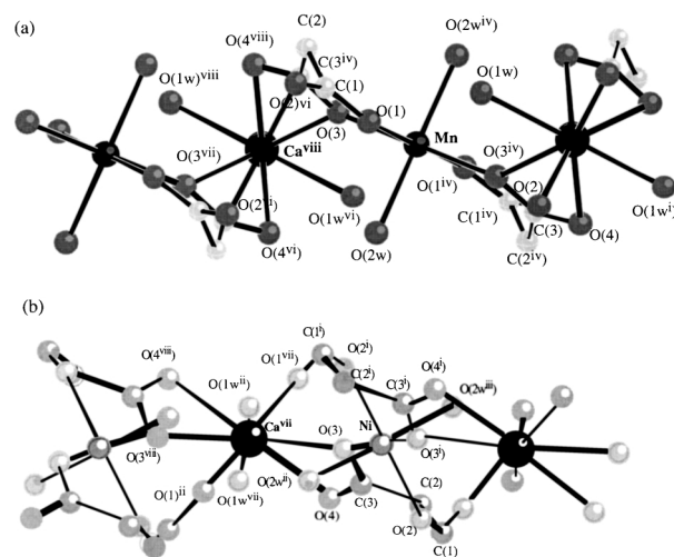
Fig. 1 Schematic representation of the atoms which form the co-ordination polyhedra for the metals in (a) [\text{CaMn}(\text{C}_3\text{H}_2\text{O}_4)_2(\text{H}_2\text{O})_4] and (b) [\text{CaNi}(\text{C}_3\text{H}_2\text{O}_4)_2(\text{H}_2\text{O})_4] \cdot 2\text{H}_2\text{O} .
