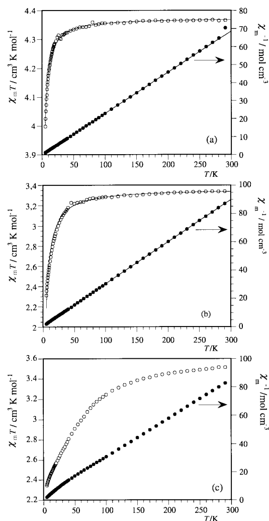
Fig. 4 Thermal evolution of \chi_m T and \chi_m^{-1} for the [\text{CaM}(\text{C}_3\text{H}_2\text{O}_4)_2(\text{H}_2\text{O})_4] compounds: \text{M} = \text{Mn} (a), \text{Fe} (b) \text{Co} (c).
