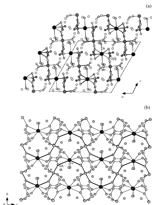
Fig. 2 Schematic representation of (a) [CaMn(C 3 H 2 O 4 ) 2 (H 2 O) 4 ] in the [0 1 0] direction and (b) [CaNi(C 3 H 2 O 4 ) 2 (H 2 O) 4 ]·2H 2 O in the bc plane.
